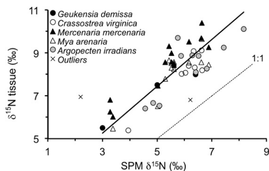
Figure 4. \delta^{15}\text{N} in bivalve tissues compared with \delta^{15}\text{N} in suspended particulate matter (SPM), separated by species (ribbed mussels ( Geukensia demissa ), oysters ( Crassostrea virginica ), quahogs ( Mercenaria mercenaria ), soft-shell clams ( Mya arenaria ), scallops ( Argopecten irradians )). Type II regression yielded a best-fit line to the combined data: y = 1.10x + 1.97 , R^2 = 0.69 , F_{47} = 103.67 , P < 0.001 . Outliers (Sokal & Rohlf 1981) were not included in the regression analysis. N-stable isotopic ratios in bivalve tissues were determined by isotope ratio mass spectrometry.
