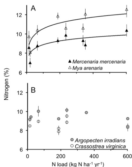
Figure 7. (A, B) Percent N in soft tissue compared with N loading rate for Cape Cod estuaries for M. mercenaria and M. arenaria (A) and A. irradians and C. virginica (B) ( M. mercenaria : y = 0.56 \ln(x) + 6.31 , R^2 = 0.61 , F_7 = 9.31 , P = 0.02 ; M. arenaria : y = 0.86 \ln(x) + 6.59 , R^2 = 0.69 , F_7 = 13.13 , P = 0.01 ). No data were available for G. demissa . Percent N was determined during mass spectrometry.
