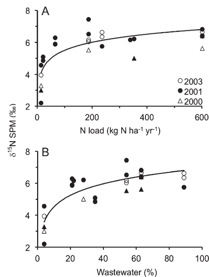
Figure 3. (A, B) \delta^{15}\text{N} in suspended particulate matter (SPM) compared with N load (A) and percent contribution of wastewater with total N load (B) for Cape Cod estuaries sampled during 1999, 2000, 2001, and 2003. (A) y = 0.73 \ln(x) + 2.16 , R^2 = 0.58 , F_{27} = 35.94 , P < 0.001 . (B) y = 1.04 \ln(x) + 2.13 , R^2 = 0.70 , F_4 = 61.04 , P < 0.001 . N-stable isotopic ratios in SPM were determined by isotope ratio mass spectrometry at either Boston University or University of California, Davis Stable Isotope Facility.
