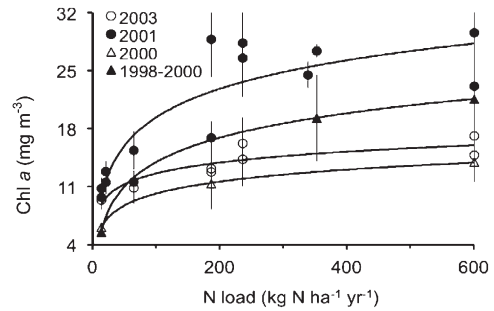
Figure 6. Mean ( \pm SE) chlorophyll a (Chl a ) concentration in near-bottom water at bivalve transplant locations 1998 to 2003 compared with N loading rates for Cape Cod estuaries. No bivalves were transplanted in 2002. For clarity, data originally reported by site were combined to yield an estuary mean for transplant sites in each year. Data for 1998 to 2000 are a 3-y average, calculated to represent conditions in Evgenidou and Valiela (2002), who reported only historical Chl a concentrations. Data from Shriver et al. (2002) and Carmichael et al. (2004) for 2001 were not significantly different ( t = -99 , df = 6 , P = 0.18 ), and were combined for simplicity. 2003: y = 1.86 \ln(x) + 3.99 , R^2 = 0.91 , F_4 = 30.84 , P = 0.01 , data from Carmichael et al. (unpubl.); 2001: y = 5.00 \ln(x) + 3.62 , R^2 = 0.90 , F_7 = 55.36 , P < 0.001 , data from Carmichael et al. (2004) and Shriver et al. (2002); 2000: y = 2.08 \ln(x) + 0.56 , R^2 = 0.99 , F_2 = 1,357.40 , P = 0.02 , data from Weiss et al. (2002); 1998 to 2000: y = 4.26 \ln(x) + 5.70 , R^2 = 0.99 , F_2 = 65,659,515.89 , P < 0.001 , data from Valiela et al. (unpubl.).
