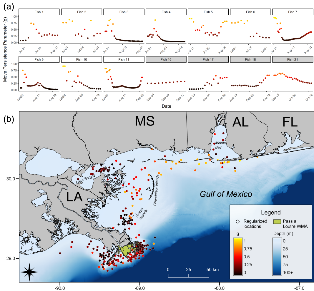
FIGURE 2 (a) The move persistence parameter ( g ), displayed as a time-series for the state-space model filtered tarpon data, with white and grey name templates indicating fish tagged in Alabama versus Louisiana, respectively. (b) Map displaying the move persistence parameter ( g ) for each of the state-space model filtered tarpon locations
